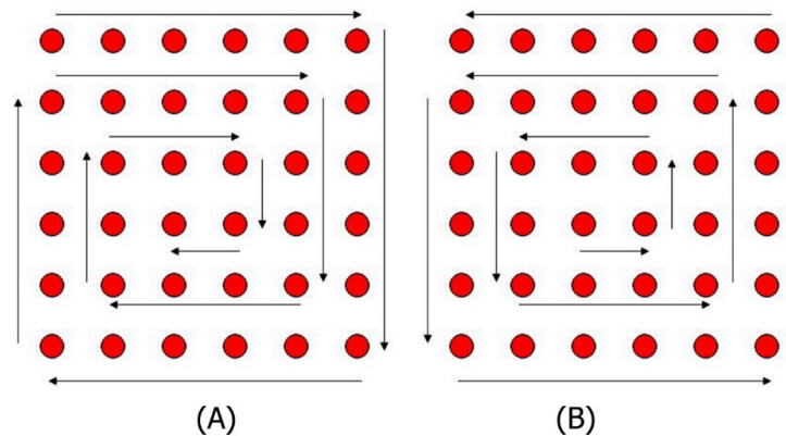
Fig. (1). (A) Forward Snail tour in matrix 6×6 (B) Backward Snail tour in matrix 6×6.
